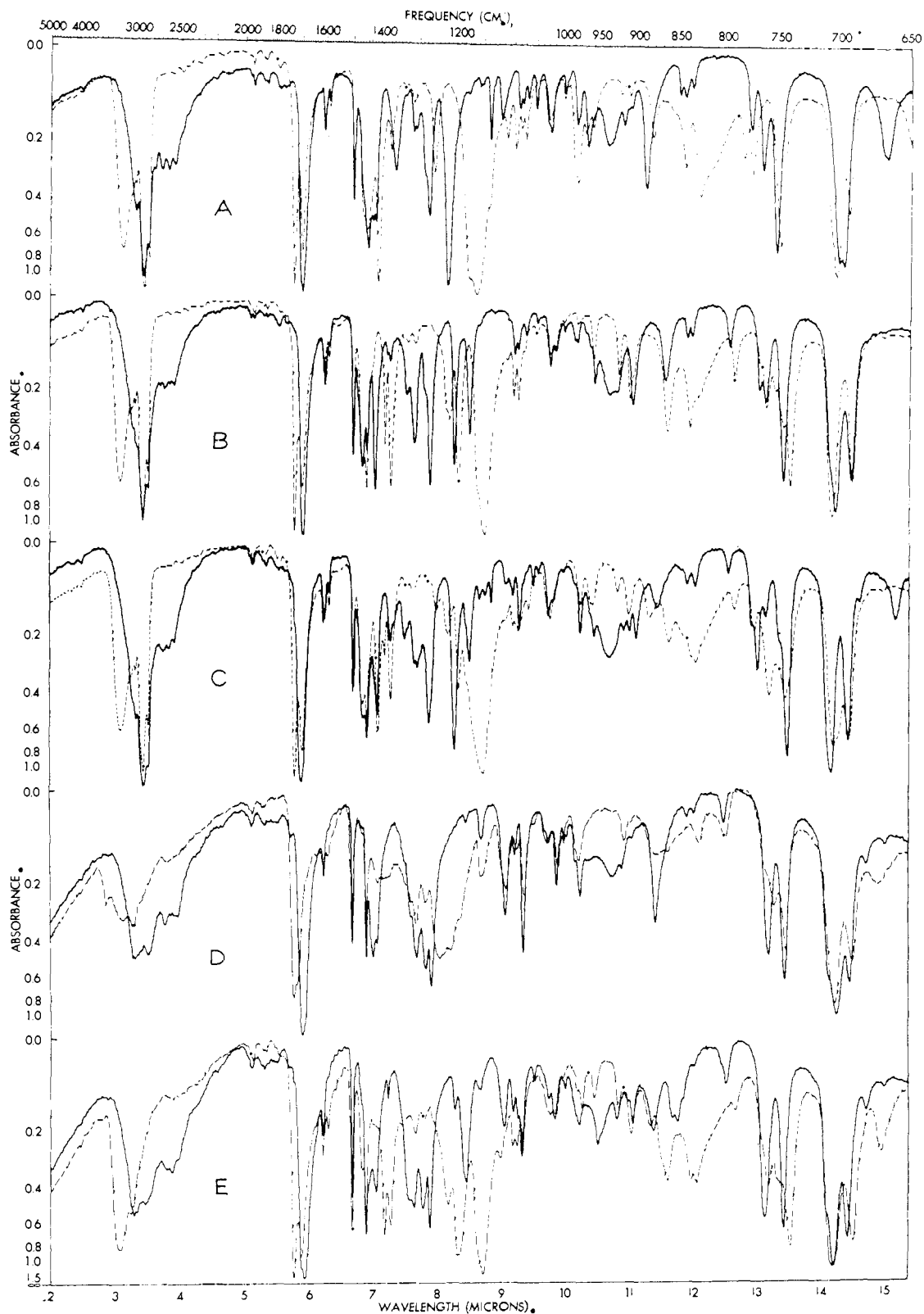
Fig. 4.--Infrared spectra: A, ( \pm )- and ( - )-2,2-diphenylcyclopropanecarboxylic acid (I) (solid line ( \pm ), dotted line ( - )); B, ( \pm )- and ( - )-1-methyl-2,2-diphenylcyclopropanecarboxylic acid (II) (solid line ( \pm ), dotted line ( + )); C, quasi-racemate (+)-I (+)-II (solid line) and solid solution ( - )-I (+)-II (dotted line); D, ( \pm )- and (+)-1-bromo-2,2-diphenylcyclopropanecarboxylic acid (III) (solid line ( \pm ), dotted line ( + )); E, quasi-racemate (+)-II ( - )-III (solid line) and solid solution (+)-II (+)-III (dotted line). A, B, and C are from mineral oil mulls over entire wave length range. D and E are Fluorolube mulls above 1334\text{ cm.}^{-1} and mineral oil mulls below 1334\text{ cm.}^{-1} .
